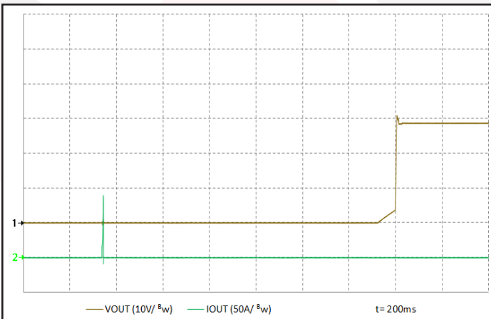
Figure 17: Rise of output voltage when a short circuit across the output terminals is removed after 30 seconds. See Figure E. R_{short} = 5\text{ m}\Omega , zero output capacitance. Ch1: V_{out} (10 V/div). Ch 2: I_{out} (50 A/div). Bandwidth: 20MHz. Timescale: 200ms/div.
