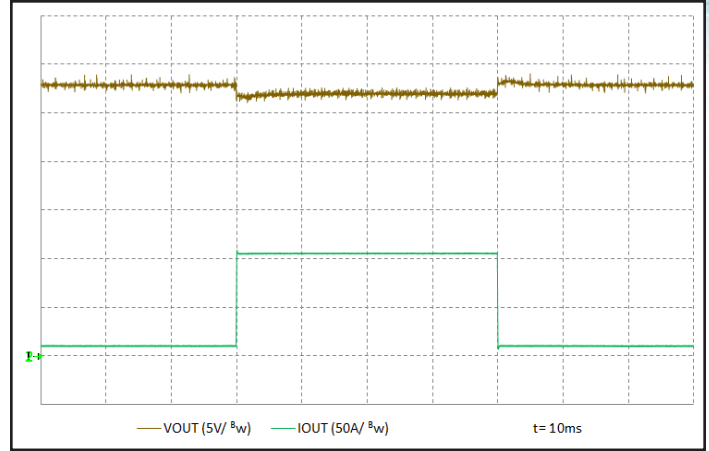
Figure 14: Output voltage response to step-change in load current 10%-100%-10% of I_{out(max)} , 470 \mu F output capacitance. Ch1: V_{out} (5 V/div). Ch 2: I_{out} (50 A/div). Bandwidth: 20 MHz. Timescale: 10.0ms/div.
