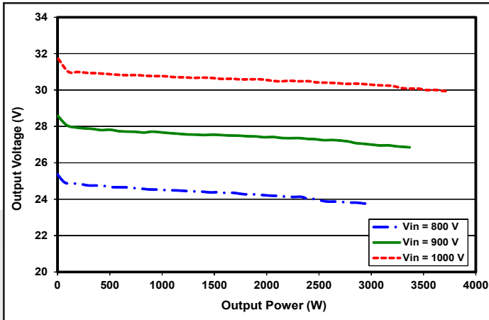
Figure 7: Output voltage vs. output power, regulation curves for minimum, nominal, and maximum input voltage at T_{CASE}=25^{\circ}C .
