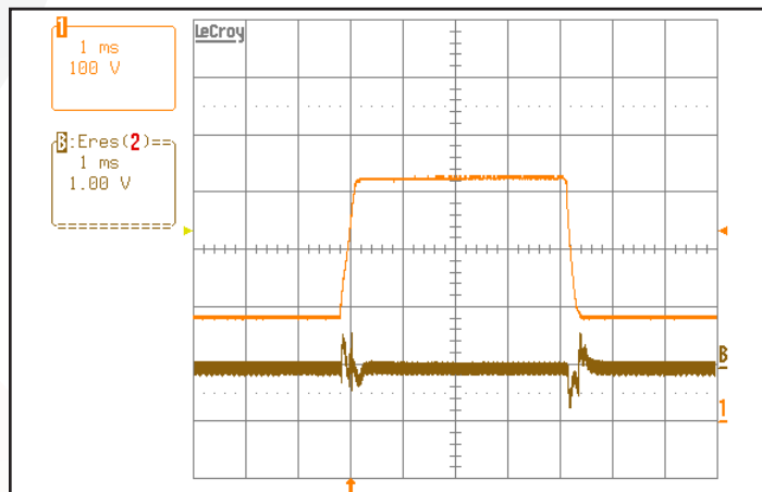
Figure 12: Output voltage response to step-change in input voltage (250V/ms). Load cap: 1μF ceramic capacitor and 10μF tantalum capacitor. Ch 1: Vin (100 V/div), Ch 2: Vout (1 V/div).
