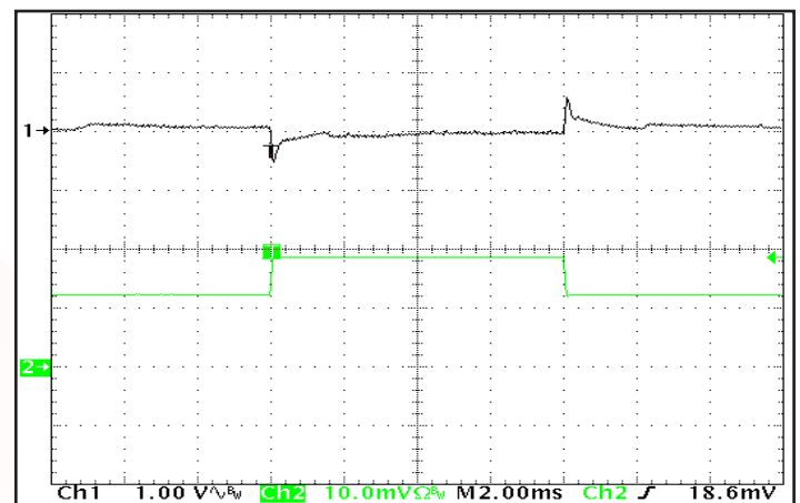
Figure 12: Output voltage response to step-change in load current (300W-450W-300W); di/dt = 0.1 \text{ A}/\mu\text{s} . Load cap: 100uF, 1 uF ceramic and 10 uF tantalum capacitors. Ch 1: Vout (1V/div), Ch 2: Iout (5A/div), (2ms/div).
