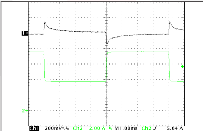
Figure 11: Output voltage response to step-change in load current 50%-100%-50% of Iout (max); dI/dt = 0.07 \text{ A}/\mu\text{s} . No external load capacitance. Ch 1: Vout (200 mV/div). Ch 2: Iout (2 A/div). (1 ms/div).
