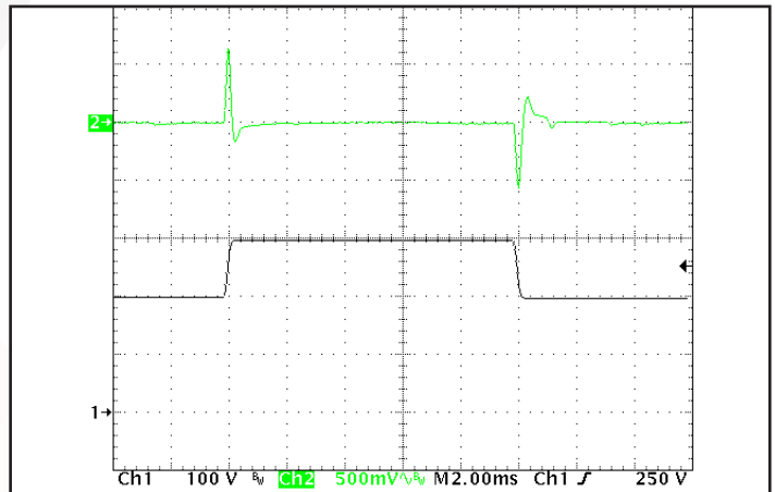
Figure 12: Output voltage response to step-change in input voltage (200 V - 300 V - 200 V); dV/dt = 500 \text{ V}/\text{ms} . Ch 1: Vin (100 V/div). Ch 2: Vout (500 mV/div). (2 ms/div).
