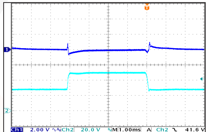
Figure 12: Output Voltage Response to Step-Change in Input Voltage, ( dV/dt = 250\text{V/ms} ). Load cap: 100 \mu\text{F} electrolytic output capacitance. Ch 1: Vout (2V/div); Ch 2: Vin (20V/div). Timescale: 1.00ms/div.
