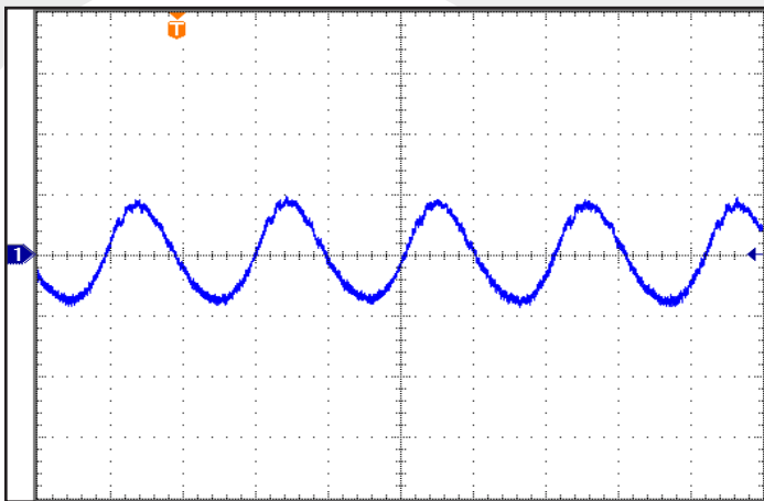
Figure 9: Input Terminal Current Ripple, i_C , at full rated output current and nominal input voltage with a 470 \mu\text{F} electrolytic capacitor (1A/div). Bandwidth: 20 MHz. Timescale: 2.00 \mu\text{s} /div. See Figure 13.
