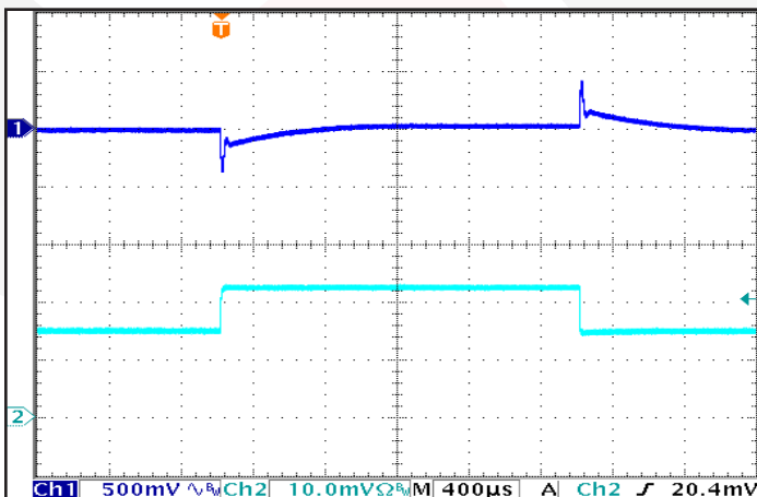
Figure 11: Output Voltage Response to Step-Change in Load Current, (50%-75%-50% of I_{\text{out(max)}} ; dI/dt = 5\text{A}/\mu\text{s} ). Load cap: 1 \mu\text{F} ceramic and 100 \mu\text{F} electrolytic capacitors. Ch 1: Vout (500mV/div); Ch 2: Iout (20A/div). Timescale: 400 \mu\text{s} /div.
