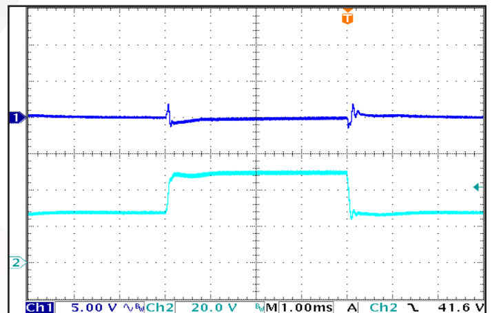
Figure 12: Output Voltage Response to Step-Change in Input Voltage , (250 V/ms). Load capacitance: 1 \mu\text{F} ceramic and 100 \mu\text{F} electrolytic capacitors. Ch 1: Vout (5 V/div); Ch 2: Vin (20 V/div). Timescale: 1.00ms/div.
