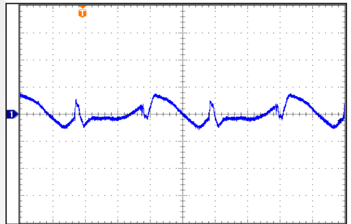
Figure 10: Output Voltage Ripple , Vout, at nominal input voltage and rated load current (100 mV/div). Load capacitance: 1 \mu\text{F} ceramic and 100 \mu\text{F} electrolytic capacitors. Bandwidth: 20 MHz. Timescale: 2 \mu\text{s} /div. See Figure 13.
