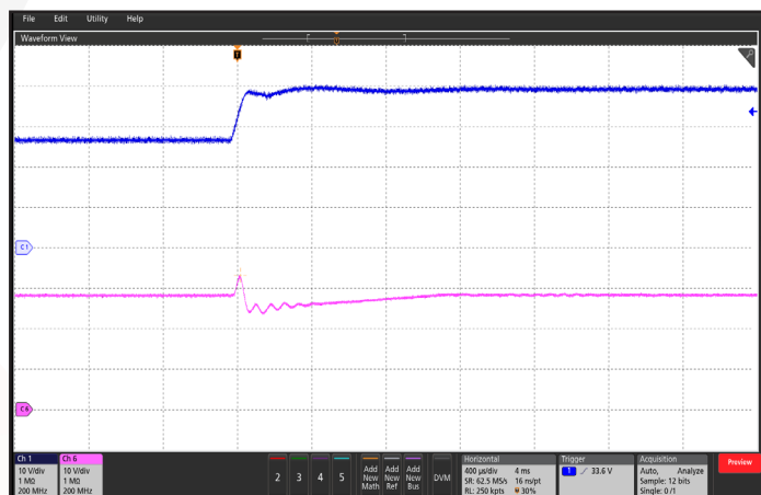
Figure 12: Output Voltage Response to Step-Change in Input Voltage, ( dV/dt = 250 V/μs ). Load capacitance: 1 μF ceramic. Ch 1: Vin (10 V/div); Ch 6: Vout (10 V/div).
