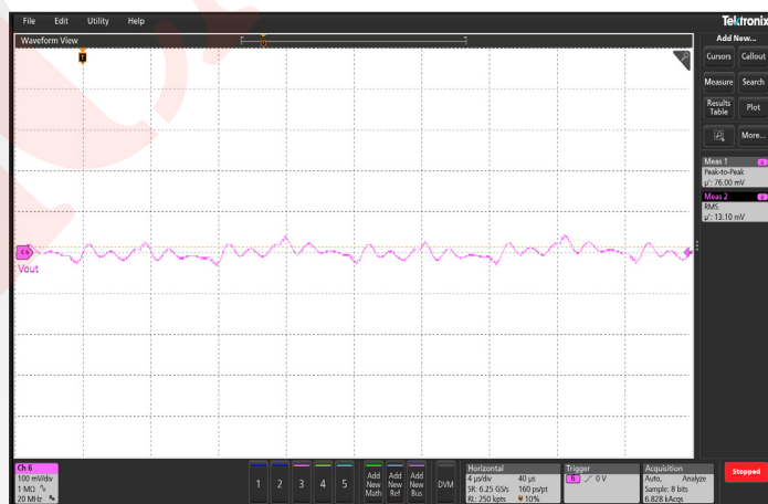
Figure 10: Output Voltage Ripple, Vout, at nominal input voltage and rated load current (100 mV/div). Load capacitance: 4 μF ceramic and 470 μF electrolytic capacitors. Timebase: 4 μs/div; Bandwidth: 20 MHz. See Figure 13.
