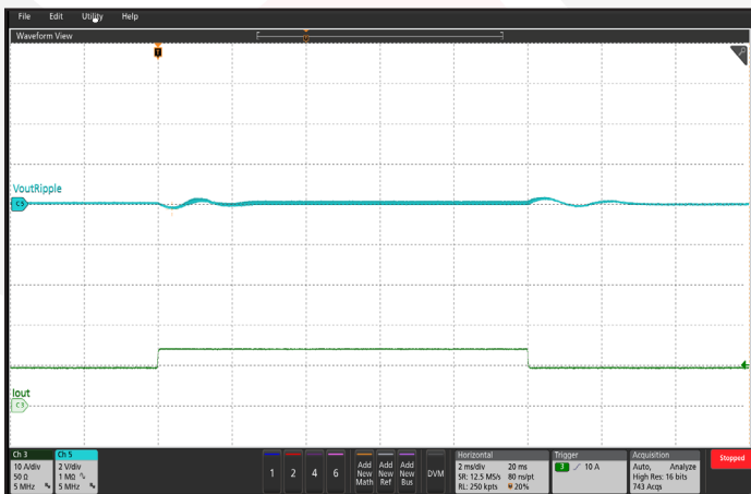
Figure 17: Hi-Cap Option Output Voltage Response to Step-Change in Load Current, (50%-75%-50% of I OUT (max); dI/dt = 10 A/μs). Load capacitance: 4 μF ceramic and 5 mF electrolytic capacitors. Ch 5: ΔV OUT (2 V/div); Ch 3: I OUT (10 A/div); Timebase: 2 ms/div
