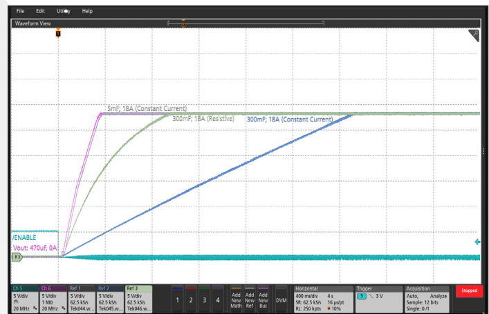
Figure 16: Hi-Cap Option Startup Waveform, input voltage pre-applied. Ch 6: V OUT , 470 μF, no load (5 V/div); Ch 5: ON/OFF Pin (5 V/div); Timebase: 400 ms/div; Constant-current loads may significantly slow down the startup ramp when combined with large capacitances.
