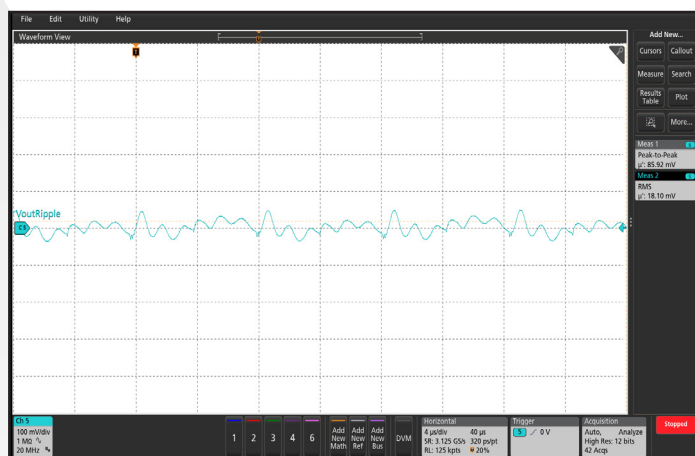
Figure 10: Output Voltage Ripple, V_{out} , at nominal input voltage and rated load current (100 mV/div). Load capacitance: 4 \mu\text{F} ceramic and 470 \mu\text{F} electrolytic capacitors. Timebase: 4 \mu\text{s}/\text{div} ; Bandwidth: 20 MHz. See Figure 13.
