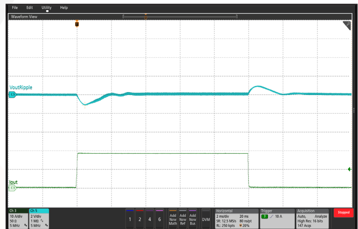
Figure 18: Hi-Cap Option Output Voltage Response to Step-Change in Load Current, (0%-100%-0% of I OUT (max); dI/dt = 10 A/μs). Load capacitance: 4 μF ceramic and 5 mF electrolytic capacitors. Ch 5: ΔV OUT (2 V/div); Ch 3: I OUT (10 A/div); Timebase: 2 ms/div
