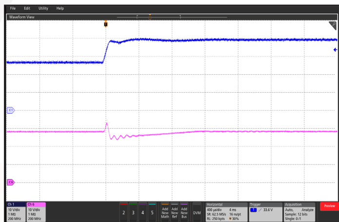
Figure 12: Output Voltage Response to Step-Change in Input Voltage, ( dV/dt = 250 \text{ V}/\text{ms} ). Load capacitance: 1 \mu\text{F} ceramic. Ch 1: Vin (10 V/div); Ch 6: Vout (10 V/div); Timebase: 400 \mu\text{s}/\text{div}
