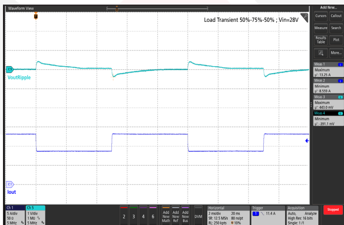
Figure 11: Output Voltage Response to Step-Change in Load Current, (50%-75%-50% of I_{out}(\text{max}) ; di/dt = 5 \text{ A}/\mu\text{s} ). Load capacitance: 4 \mu\text{F} ceramic and 470 \mu\text{F} electrolytic capacitors. Ch 1: I_{out} (5 A/div); Ch 5: \Delta V_{out} (1 V/div); Timebase: 2 ms/div
