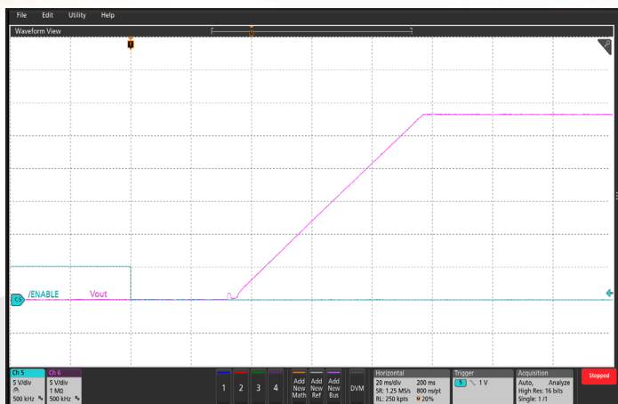
Figure 7: Typical Startup Waveform, input voltage pre-applied. Ch 5: ON/OFF Pin (5 V/div); Ch 6: Vout (5 V/div); Timebase: 20 ms/div
