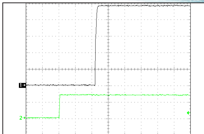
Figure 8: Turn-on transient at full resistive load and zero output capacitance initiated by V_{in} . ON/OFF Pin previously low. Ch 1: V_{out} (10V/div). Ch 2: V_{in} (20V/div).
