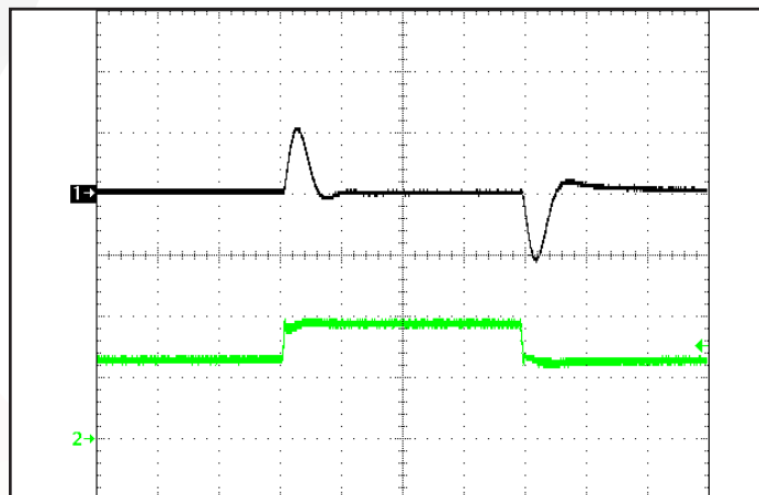
Figure 12: Output voltage response to step-change in input voltage (500V/ms) at full load current. Load cap: 100 \mu F electrolytic capacitance. Ch1: V_{out} (2V/div), Ch 2: V_{in} (20V/div).
