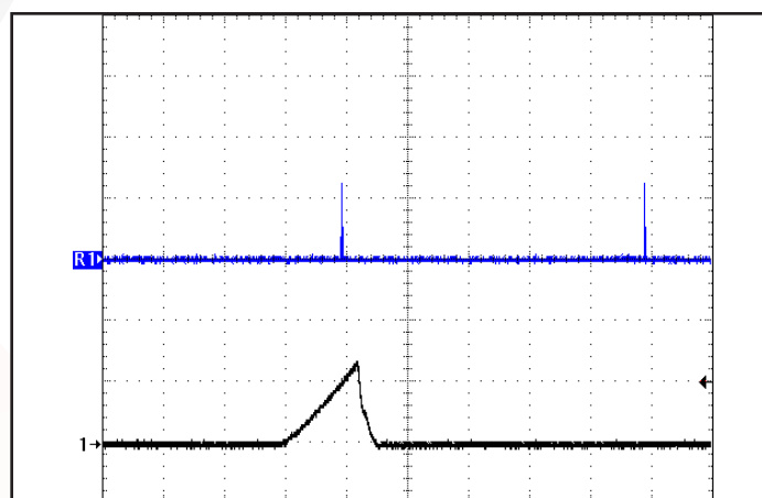
Figure 18: Load current (5A/div) as a function of time (200us/div and 40ms/div) when the converter attempts to turn on into a 10 mΩ short circuit.
