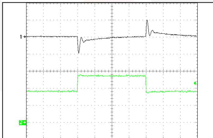
Figure 11: Output voltage response to step-change in load current (50%-75%-50% of I_{out(max)} ; dI/dt = 0.1 A/ \mu s). Load cap: 1 \mu F ceramic capacitor. Ch 1: V_{out} (2V/div), Ch 2: I_{out} (1A/div).
