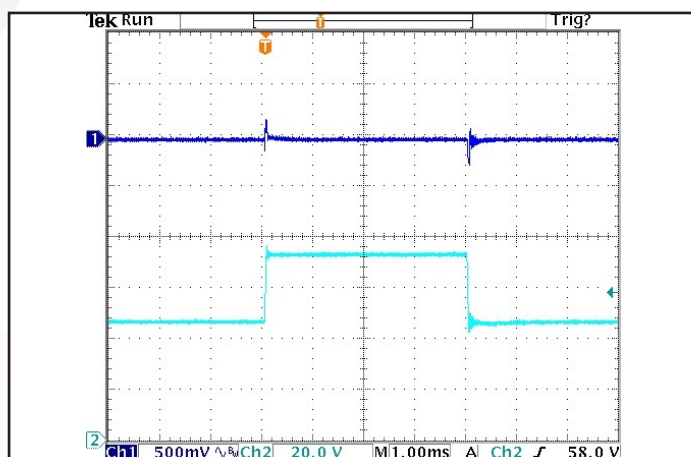
Figure 12: Output voltage response to step-change in input voltage (250V/ms). Load cap: 100 µF electrolytic output capacitance. Ch 1: Vout (500mV/div), Ch 2: Vin (20V/div).
