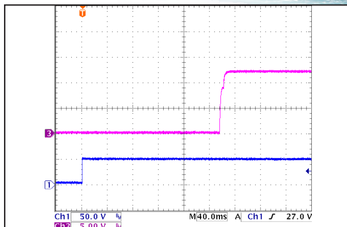
Figure 8: Turn-on transient at full resistive load and zero output capacitance initiated by Vin. ON/OFF Pin previously low. Ch 1: Vin (50V/div). Ch 3: Vout (5V/div).
