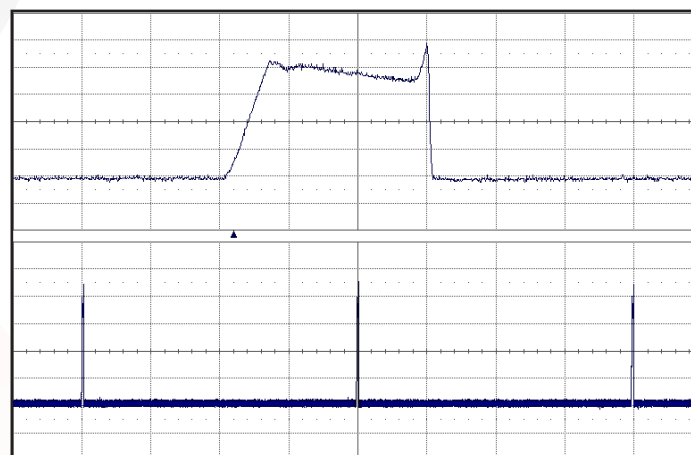
Figure 18: Load current (10A/div) as a function of time (0.5ms/div and 2ms/div) when the converter attempts to turn on into a 10 mΩ short circuit.
