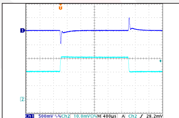
Figure 11: Output voltage response to step-change in load current (50%-75%-50% of I_{out(max)} ; dI/dt = 0.1 \text{ A}/\mu\text{s} ). Load cap: 1 µF ceramic and 15 µF tantalum capacitors. Ch 1: Vout (500mV/div), Ch 2: Iout (5A/div).
