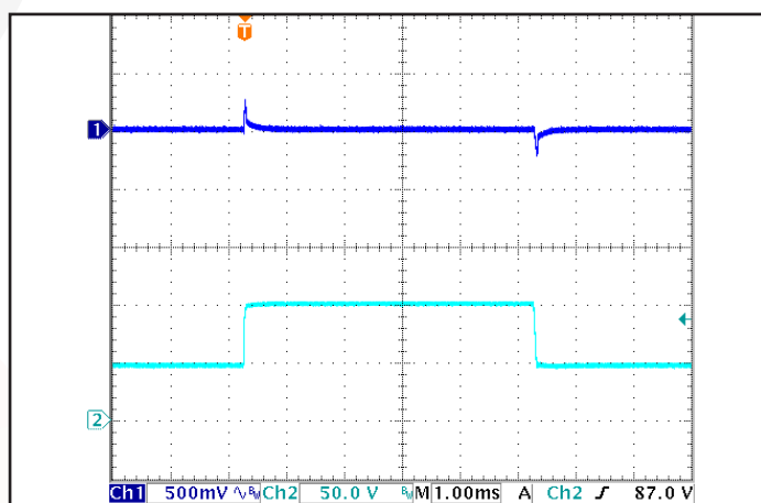
Figure 12: Output voltage response to step-change in input voltage (250V/ms). Load cap: 100 µF electrolytic output capacitance. Ch 1: Vout (500mV/div), Ch 2: Vin (50V/div).
