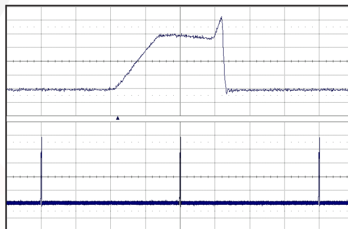
Figure 18: Load current (20A/div) as a function of time (0.5ms/div and 50ms/div) when the converter attempts to turn on into a 10 mΩ short circuit.
