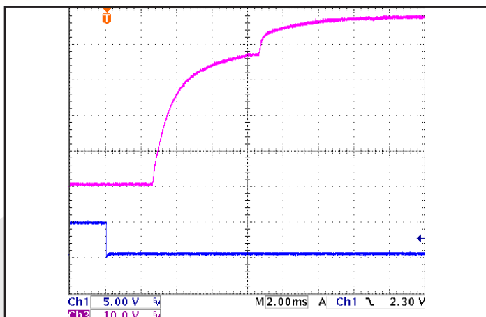
Figure 7: Typical startup waveform. Input voltage pre-applied, ON/OFF Pin. Ch 1: ON/OFF Pin (5V/div). Ch 3: Vout (10V/div), Time (2ms/div).
