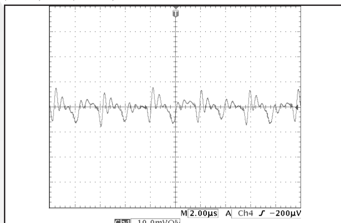
Figure 10: Output voltage ripple, Vout, at nominal input voltage and rated load current (10 mV/div), Time (2μs/div). Load capacitance: 1μF ceramic capacitor and 10μF tantalum capacitor. Bandwidth: 10 MHz. See Figure 17.
