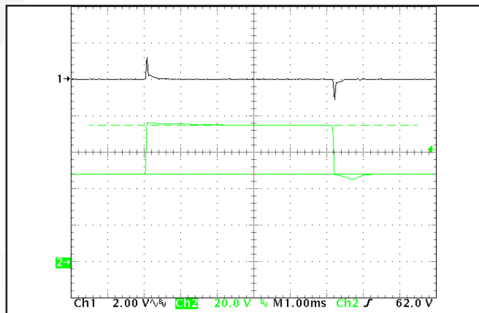
Figure 12: Output voltage response to step-change in input voltage (250V/ms). Load cap: 100 μF electrolytic output capacitance. Ch 1: Vout (2V/div), Ch 2: Vin (20V/div), Time (1ms/div).
