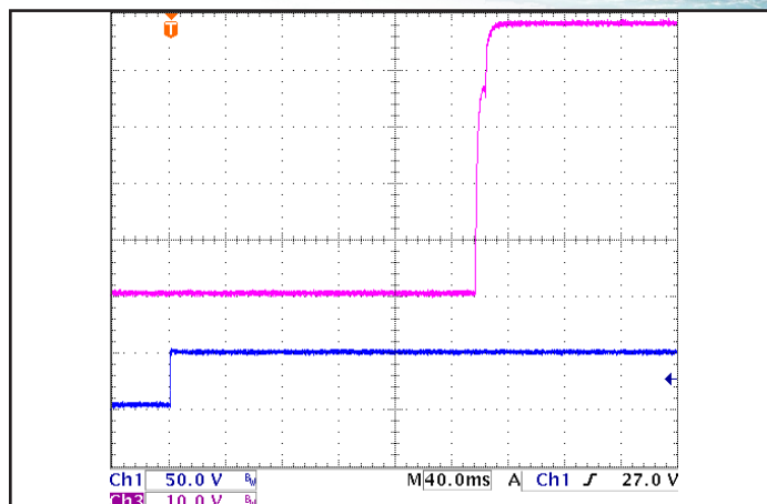
Figure 8: Turn-on transient at full resistive load and zero output capacitance initiated by Vin. ON/OFF Pin previously low. Ch 1: Vin (50V/div). Ch 3: Vout (10V/div), Time (40ms/div).
