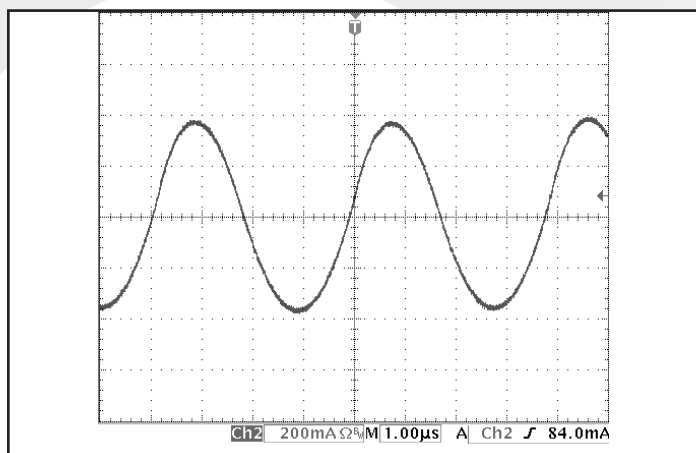
Figure 9: Input terminal current ripple, i_C , at full rated output current and nominal input voltage with SynQor MCOTS filter module (200 mA/div), Time (1μs/div). Bandwidth: 20MHz. See Figure 17.
