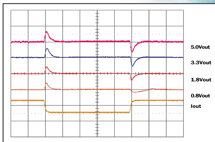
Figure 8: Output voltage response for 0.8V, 1.8V, 3.3V, 5.0V units to step-change in load current (50-75-50% of Iout max; di/dt=0.1A/μs). Load cap: 100 μF, 100mΩ ESR tant, 22 μF cer. Ch 1: Iout (10A/div), Ch 2-5: Vout (500mV/div). 200μs/div.
