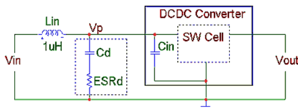
Figure B: Converter with Input Filter.
