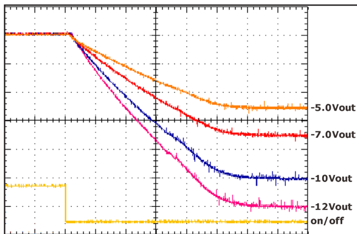
Figure 6: Turn-on transient at full load (resistive load) (10 ms/div). Ch 1: ON/OFF input (2V/div), Ch 2-5: Vout (2V/div)
