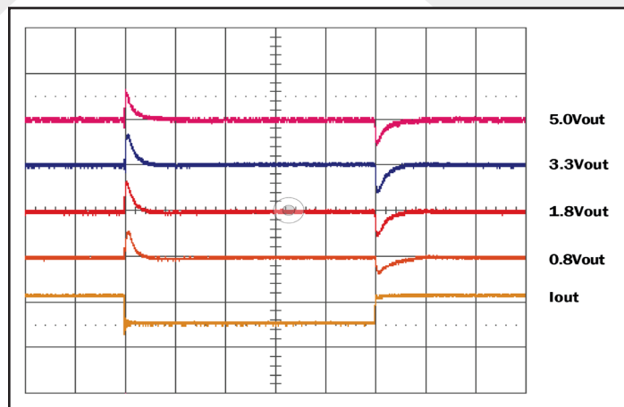
Figure 9: Output voltage response for 0.8V, 1.8V, 3.3V, 5.0V units to step-change in load current (50-75-50% of Iout max; di/dt=3A/μs). Load cap: 100 μF, 100mΩ ESR tant, 22 μF cer. Ch 1: Iout (10A/div), Ch 2-5: Vout (500mV/div). 200μs/div.
