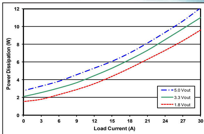
Figure 2: Power dissipation at positive output voltage vs. load current for nominal input voltage at 25°C.
