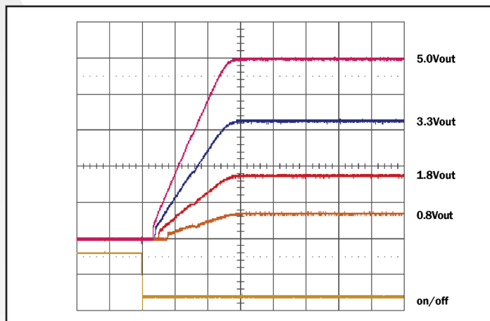
Figure 4: Turn-on transient at full load (resistive load) (2 ms/div). Ch 1: ON/OFF input (5V/div), Ch 2-5: Vout (1V/div)
