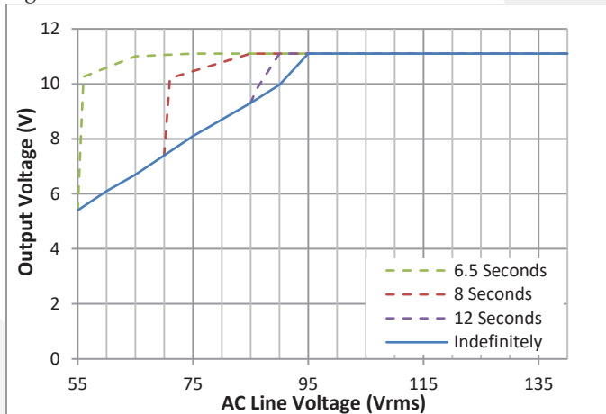
Figure 8: Full Load Output Voltage during Line Brownouts
