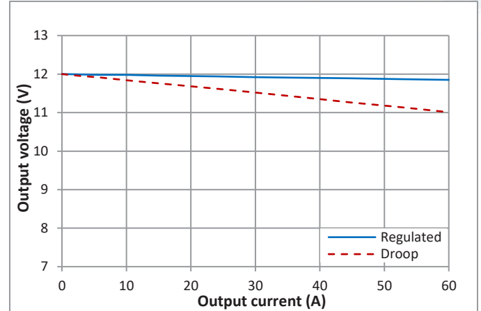
Figure 9: Steady-State Output Voltage vs. Output Current characteristics for both Regulated and Controlled Droop models.
