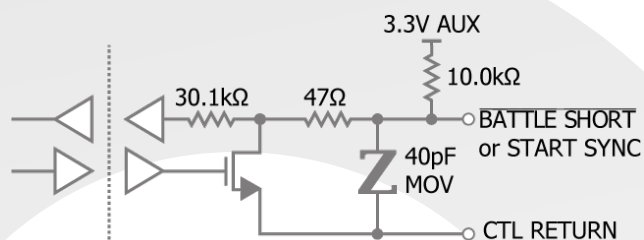
Figure 23: Internal circuitry for BATTLE SHORT and START SYNC pins.
