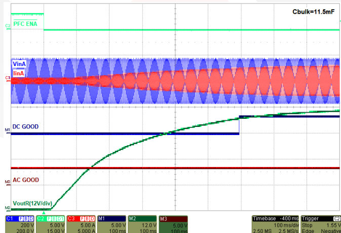
Figure 19: Timing from PFC ENA to startup and DC GOOD, VinA and IinA also shown for reference.
