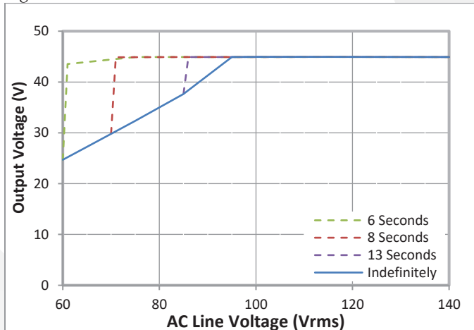
Figure 8: Full Load Output Voltage during Line Brownouts
