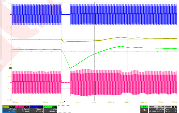
Figure 10: Line drop out with 600µF hold-up capacitor at full load (115Vrms, 400Hz) Ch1: Vout (10V/div), Ch2: Iin (10A/div), Ch3: Vin (200V/div), Ch4: Vhold-up (100V/div), Timebase: (100ms/div).
