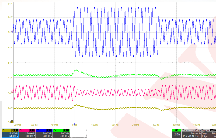
Figure 7: Input transient with 600µF hold-up capacitor at full load (115Vrms-220Vrms-115Vrms, 60Hz) Ch1: Vout (10V/div), Ch2: Iin (20A/div), Ch3: Vin (200V/div), Ch4: Vhold-up (100V/div), Timebase: (100ms/div).
