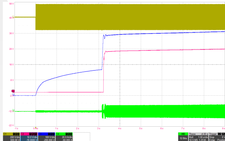
Figure 4: Typical startup waveform with 600µF hold-up capacitor (115Vrms, 400Hz) Ch1: Vin (200V/div), Ch2: Vout (10V/div), Ch3: Hold-up capacitor voltage (100V/div), Ch4: Iin (20A/div), Timebase: (1s/div).
