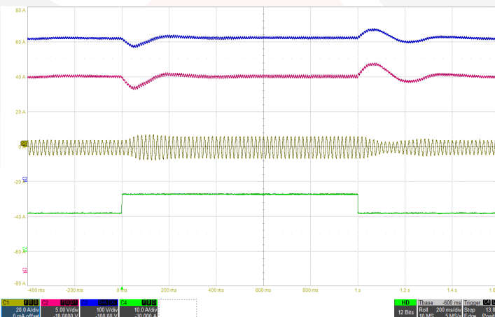
Figure 5: Load transient with 600µF hold-up capacitor (50%-75%-50% of I_{max} , 115Vrms, 60Hz) Ch1: Iin (20A/div), Ch2: Vout (5V/div), Ch3: Hold-up capacitor voltage (100V/div), Ch4: Iout (10A/div), Timebase: (200ms/div).
