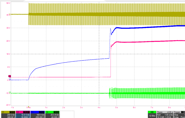
Figure 3: Typical startup waveform with 600µF hold-up capacitor (115Vrms, 60Hz) Ch1: Vin (200V/div), Ch2: Vout (10V/div), Ch3: Hold-up capacitor voltage (100V/div), Ch4: Iin (20A/div), Timebase: (1s/div).
