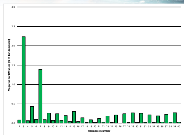
Figure 20: Input current harmonic components at full load, 115Vrms 400 Hz, T=25°C (Tested with MPFIC module and MACF-400-230-HT filter).
