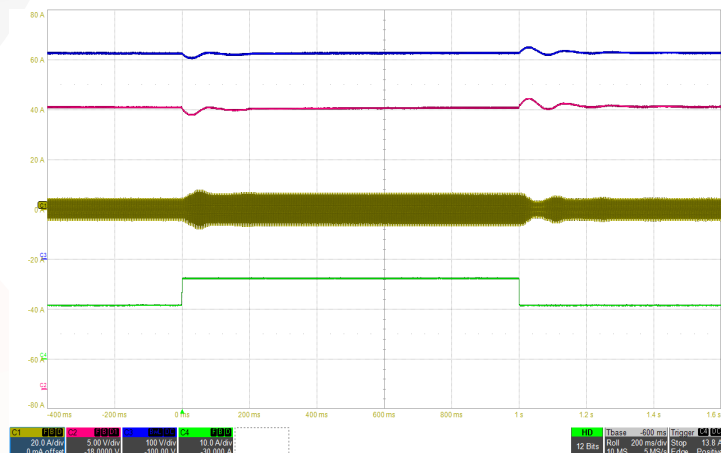
Figure 6: Load transient with 600µF hold-up capacitor (50%-75%-50% of I_{max} , 115Vrms, 400Hz) Ch1: Iin (20A/div), Ch2: Vout (5V/div), Ch3: Hold-up capacitor voltage (100V/div), Ch4: Iout (10A/div), Timebase: (200ms/div).
