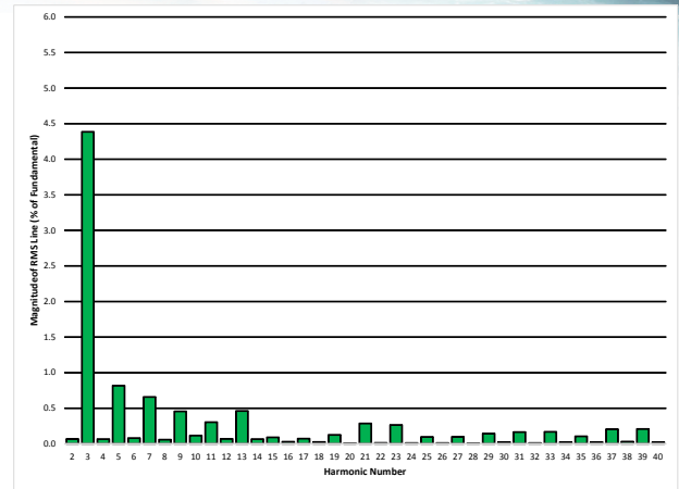
Figure 20: Input current harmonic components at full load, 115Vrms 400 Hz, T=25^{\circ}\text{C} (Tested with MPFIC module and MACF-400-230-HP filter).
